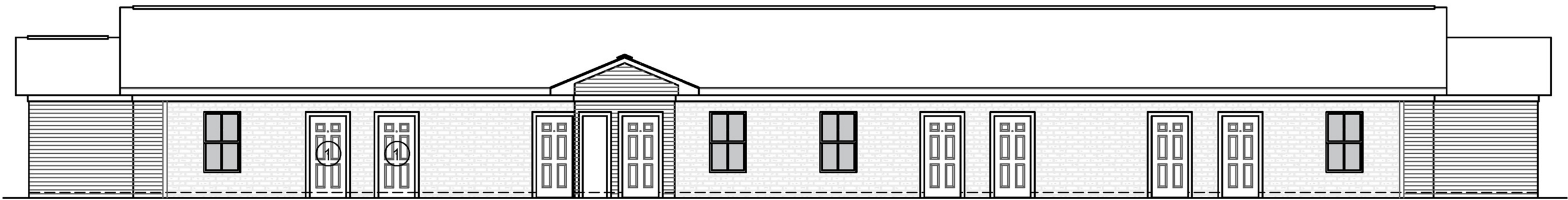
BLDG A & F REGULAR UNITS BACK ELEVATION
