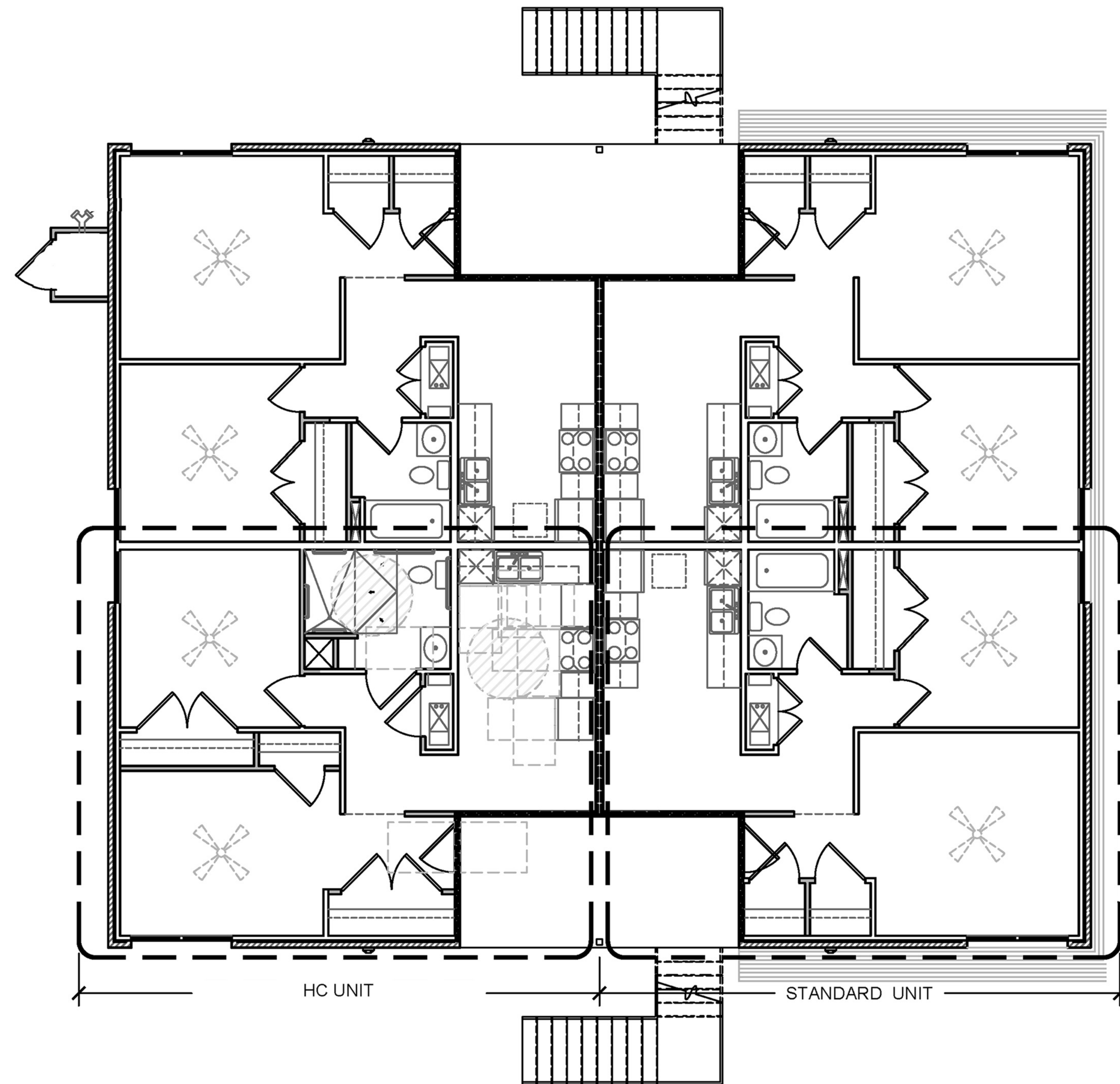
BLDGS A & B (1-BED/1-BATH UNITS) FIRST FLOOR PLAN (SECOND FLOOR SIMILAR)
