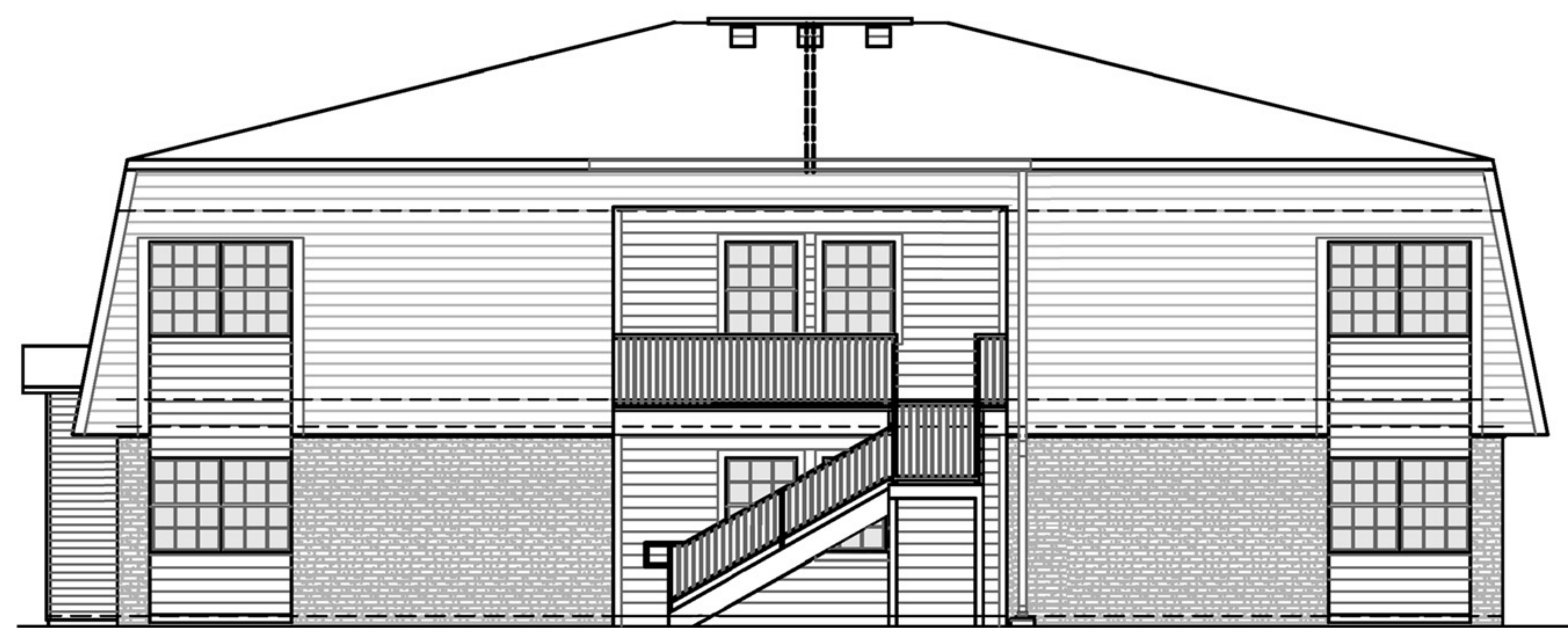
BLDGS A & B (1-BED/1-BATH UNITS) FRONT & REAR ELEVATION
